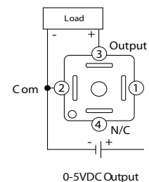
0-5VDC Output
