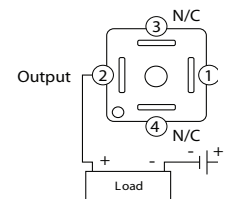
4-20mA Output
