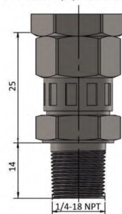
1/4"-18NPT (M) swivel adapter
