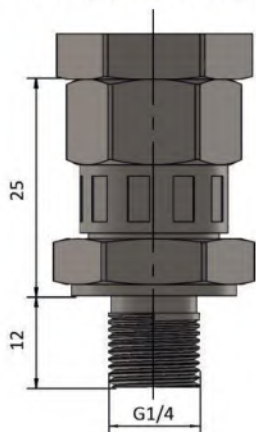
1/4"G (M) swivel adapter
